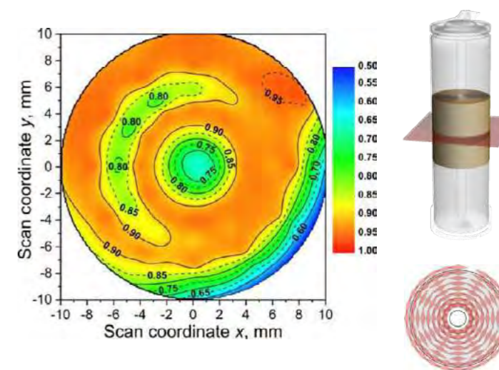
Figure 4: Lithium concentration in the graphite anode of charged Li-ion cell (type 18650) determined using spatially-resolved diffraction of thermal neutrons along the cut described by the right figures. Top: Investigated volume. Bottom: Distribution of gauge volumes.
